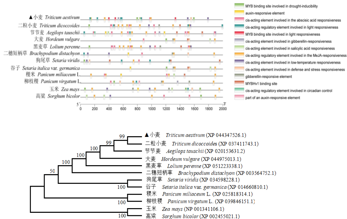
Fig.S1 Cloning of TaMYBS1-like genes
